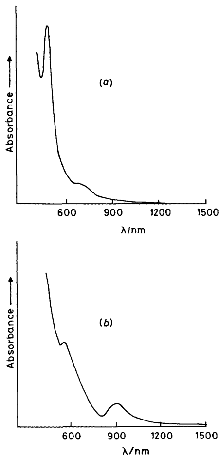
Figure 2. Electronic absorption spectra ( 1 \times 10^{-3} \text{ mol dm}^{-3} dichloromethane solution) of (a) [\text{Re}_2\text{Cl}_3(\text{dppe})_2(\text{CNBU}^t)]\text{PF}_6 and (b) [\text{Re}_2\text{Cl}_3(\text{dppe})_2(\text{CNBU}^t)][\text{PF}_6]_2
